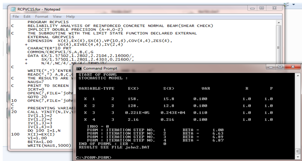
Fig. 12: Reliability Analysis using FORM5 for limit state in shear
