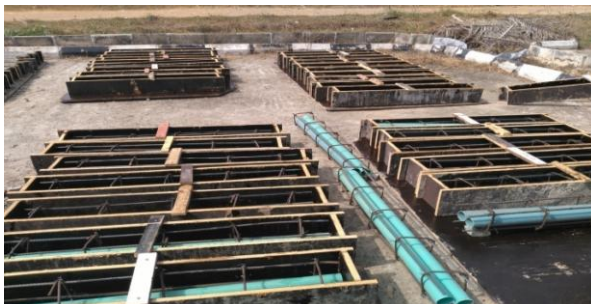
Fig. 6: Beam formwork with and without PVC pipes
