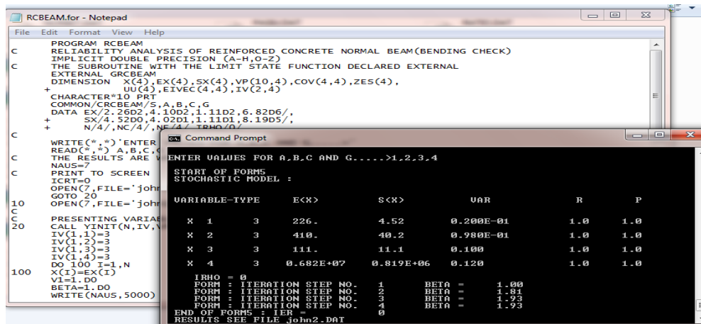
Fig. 11: Reliability Analysis using FORM5 for limit state in bending
