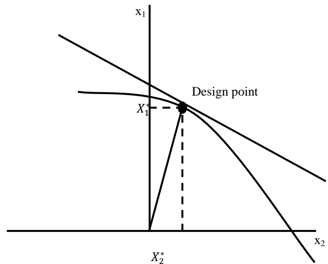
Fig. 1: Hasofer – lind reliability index
